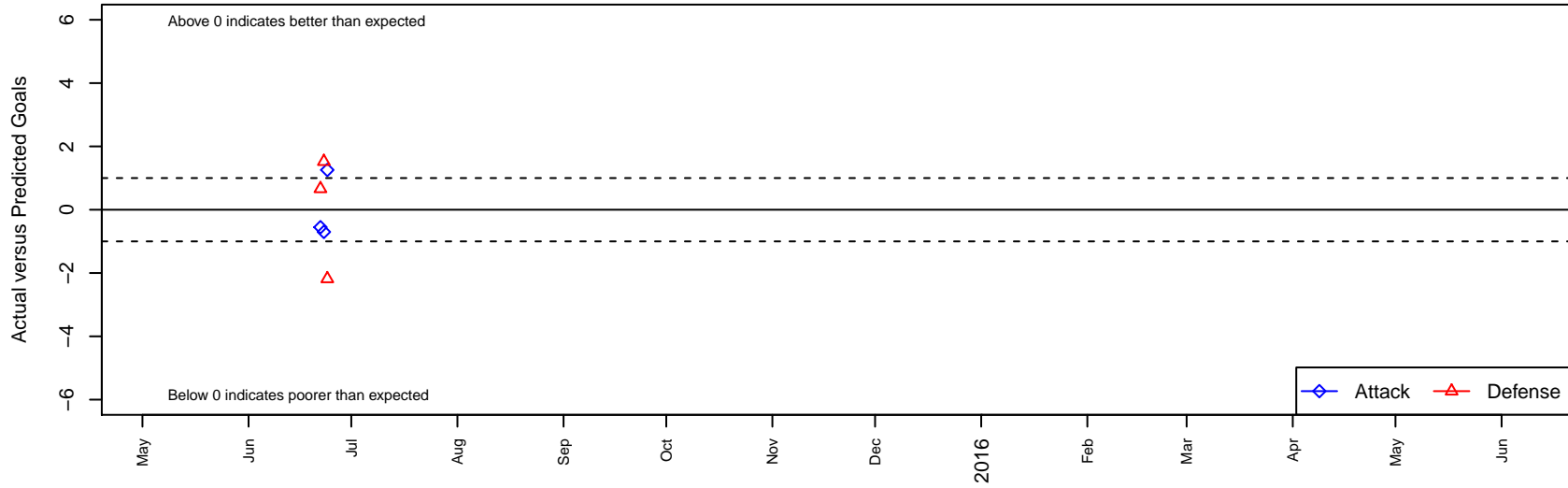
Arizona Arsenal Premier 97 Teal B96 Dots are actual minus expected GF (blue circles) and GA (red triangles). Blue line is smoothed change in attack strength. Red is smoothed change in defense strength.
